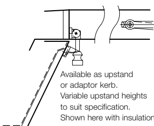
XL 123 Hinged Access
